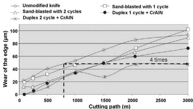
Fig. 6. Wear of the edges versus the cutting path in micro-peeling of beech.
